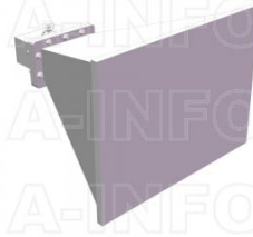
LB-510-15-C-7/16FSP0 Standard Gain Horn Antenna 1.45-2.2GHz 15dB Gain 7/16(DIN) Female
